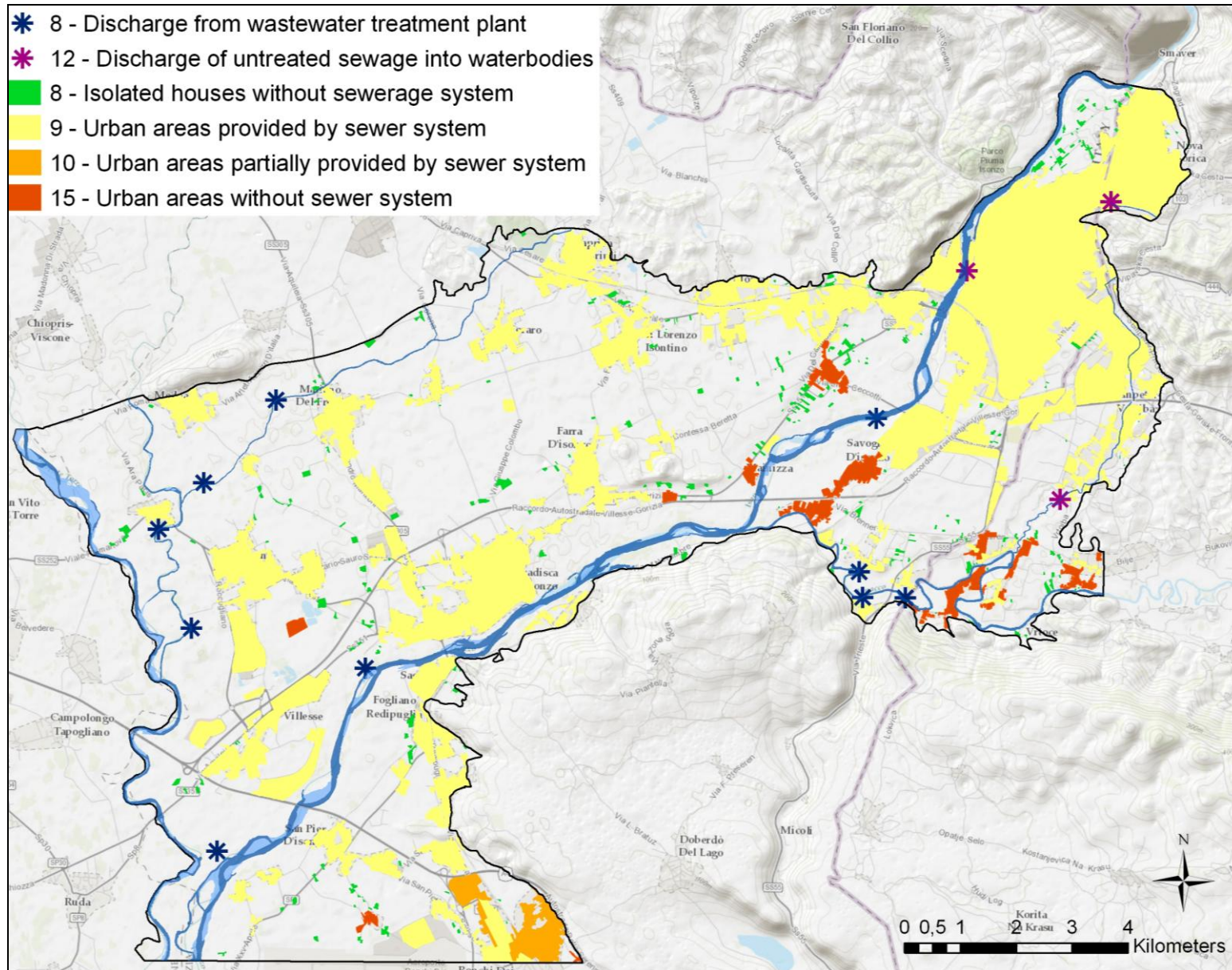
Classification of urban areas according to increasing hazard (from green to red) based on the potential pollution from municipal wastewater. The discharge of wastewater treatment plants (blue asterisk) and of untreated sewage (purple asterisk) are also reported.
